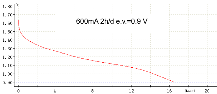
Chart 1. Discharge diagram
