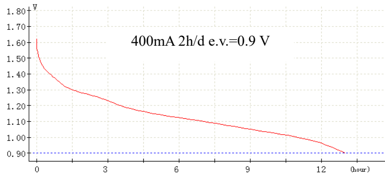
Chart 1. Discharge diagram
